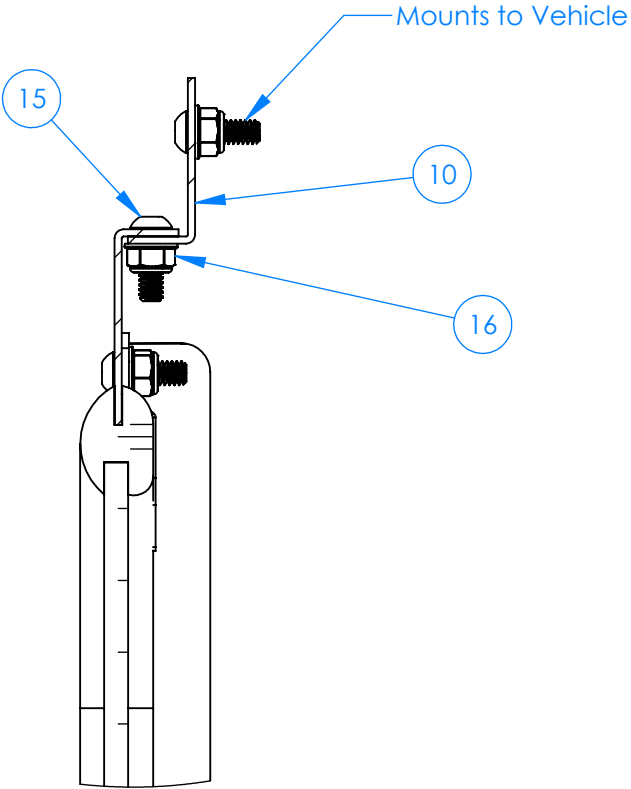
DETAIL B SCALE 1 : 2
